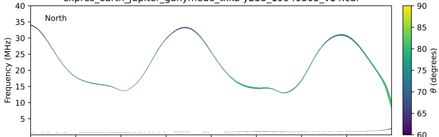
expres_earth_jupiter_ganymede_txka-y235_19940305_v14.cdf
