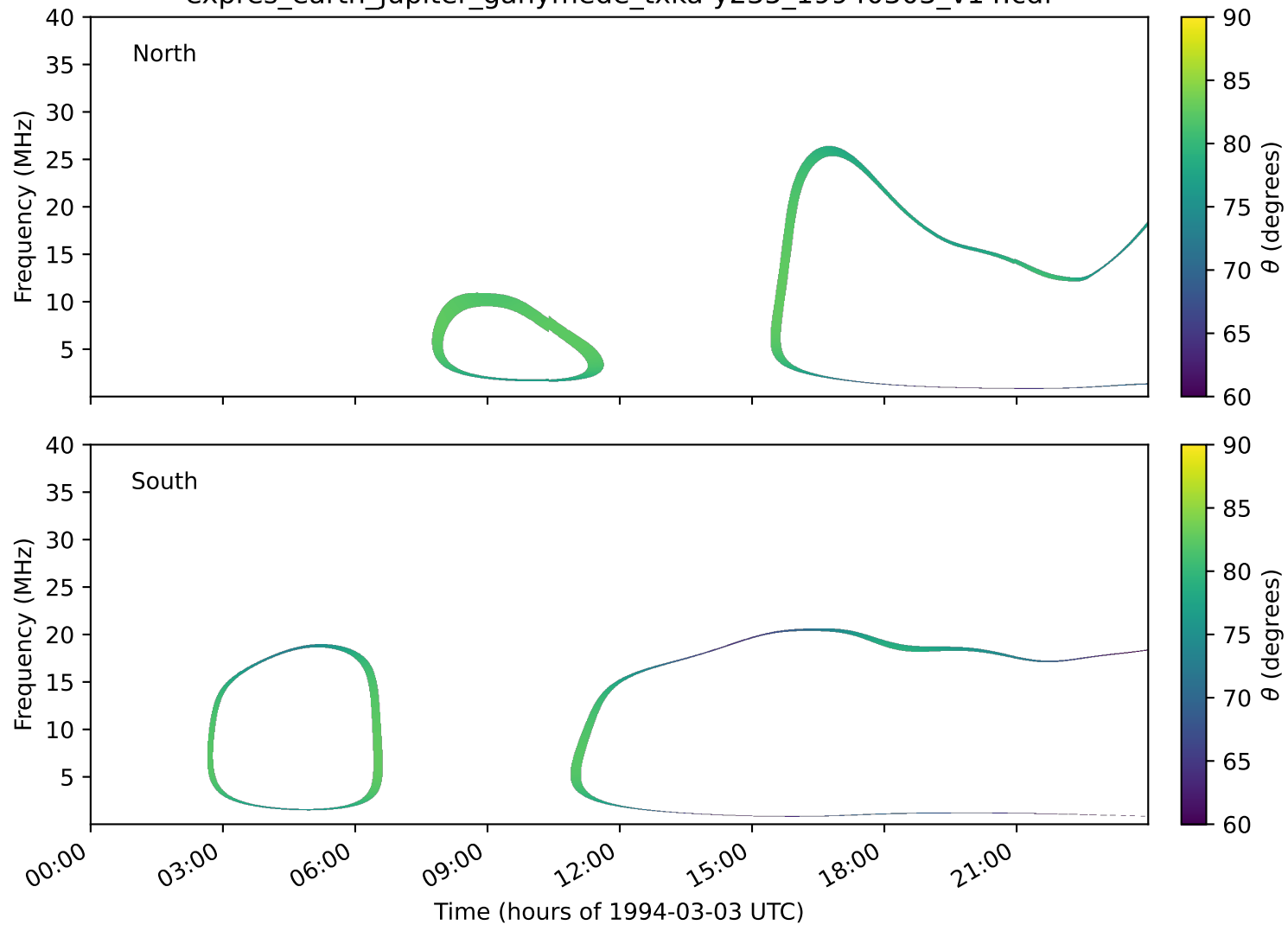
expres_earth_jupiter_ganymede_txka-y235_19940303_v14.cdf
