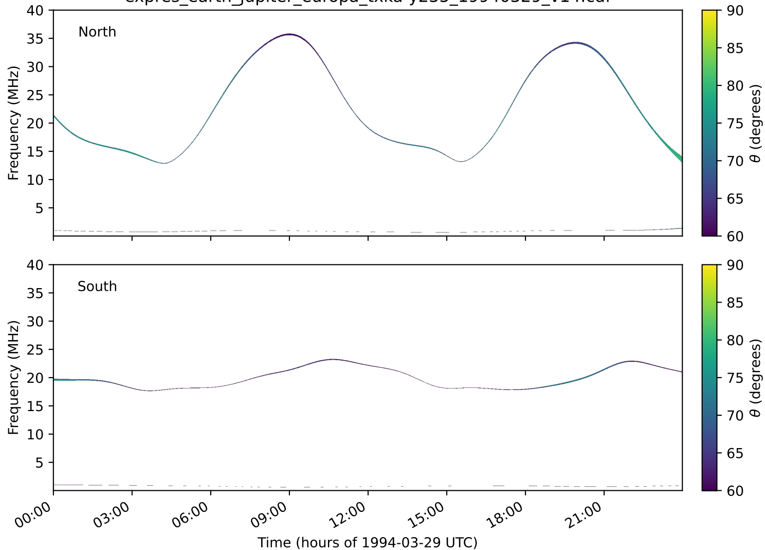
expres_earth_jupiter_europa_txka-y235_19940329_v14.cdf
