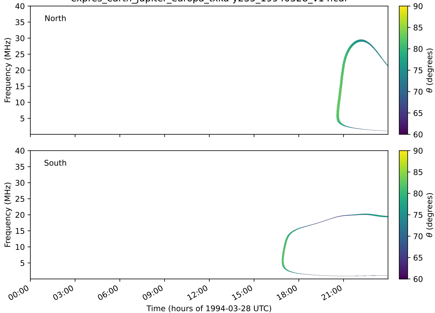
expres_earth_jupiter_europa_txka-y235_19940328_v14.cdf
