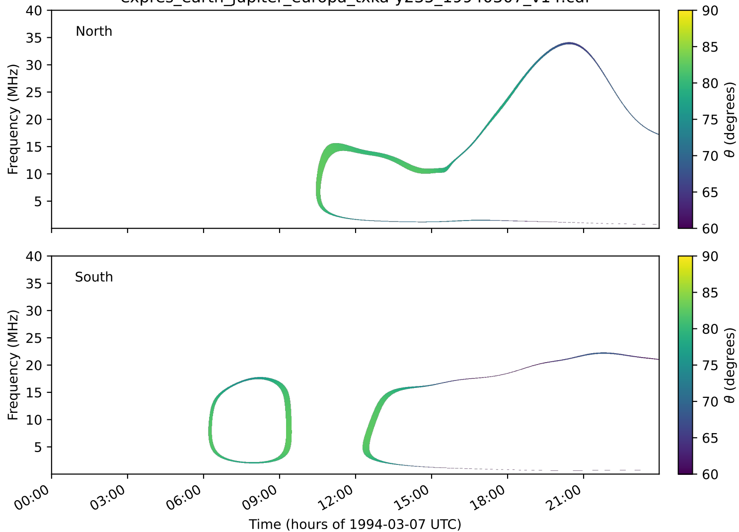
expres_earth_jupiter_europa_txka-y235_19940307_v14.cdf
