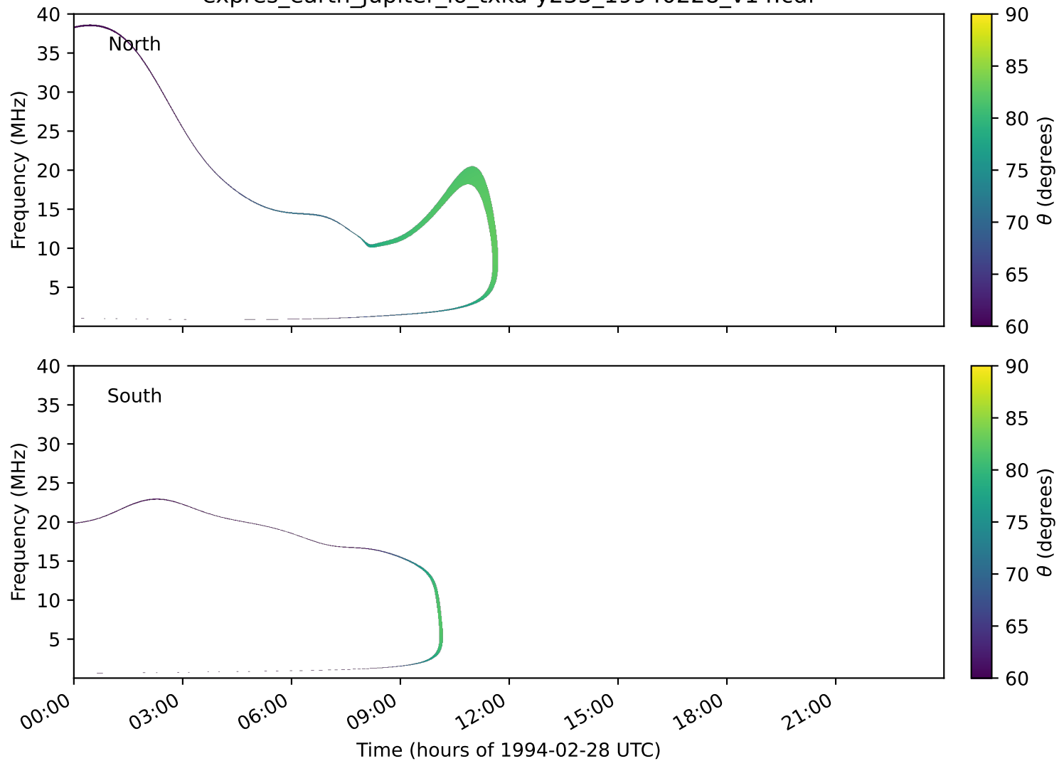
expres_earth_jupiter_io_txka-y235_19940228_v14.cdf
