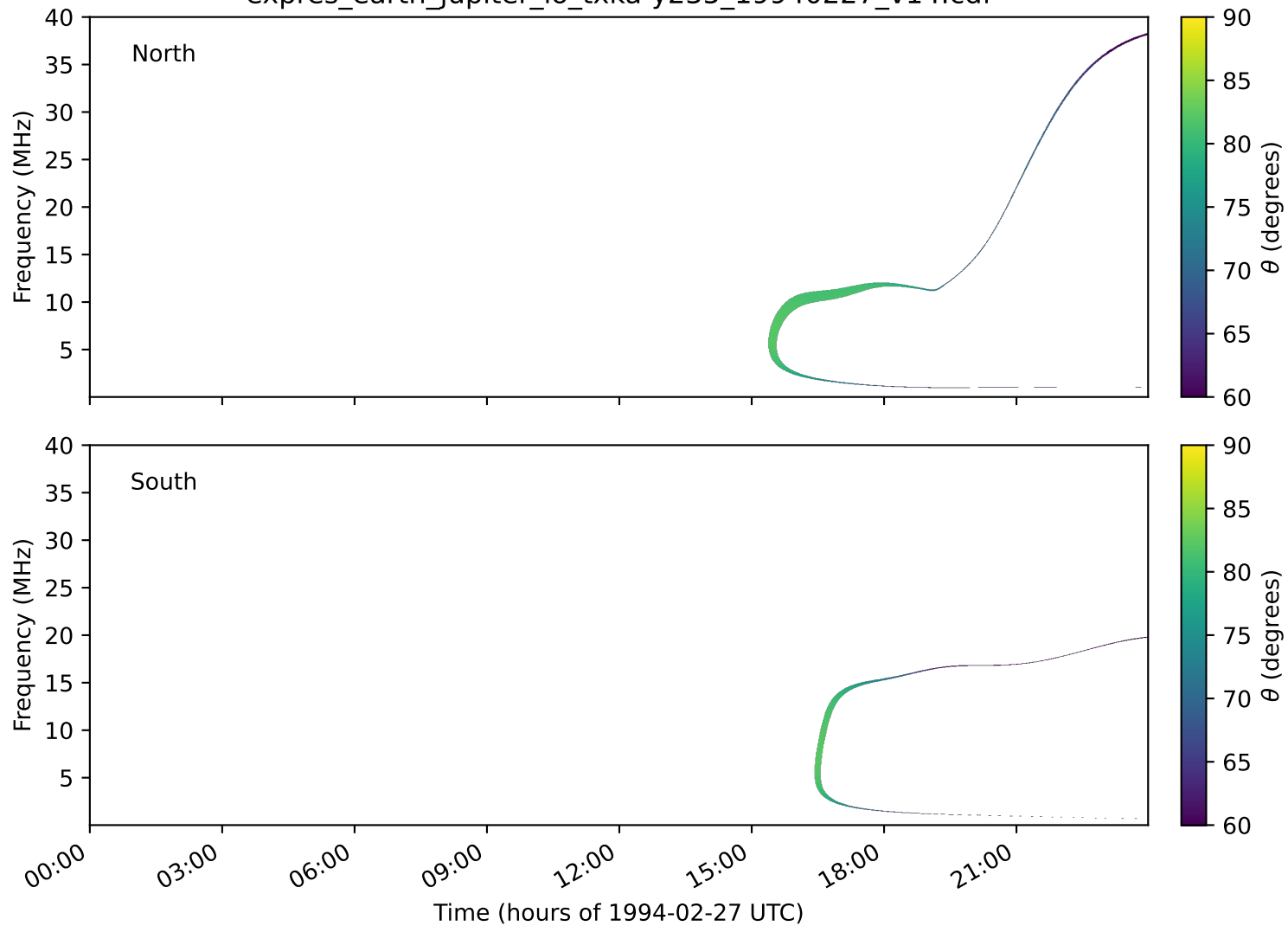
expres_earth_jupiter_io_txka-y235_19940227_v14.cdf
