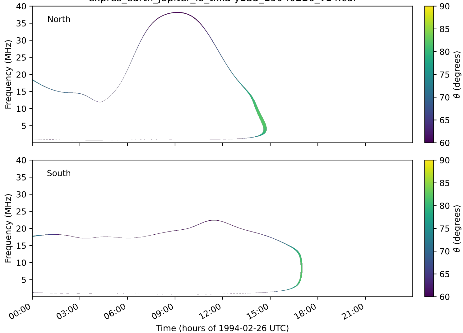
expres_earth_jupiter_io_txka-y235_19940226_v14.cdf
