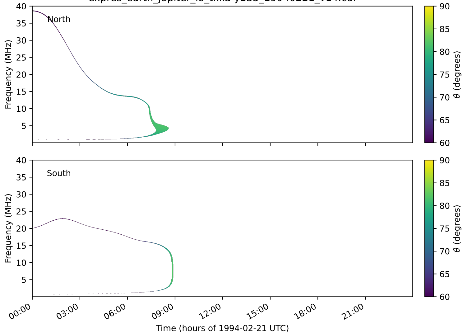
expres_earth_jupiter_io_txka-y235_19940221_v14.cdf
