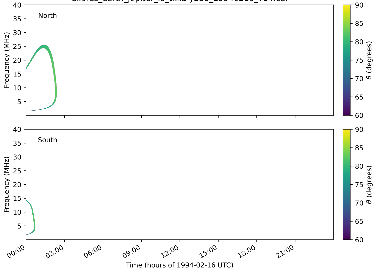
expres_earth_jupiter_io_txka-y235_19940216_v14.cdf
