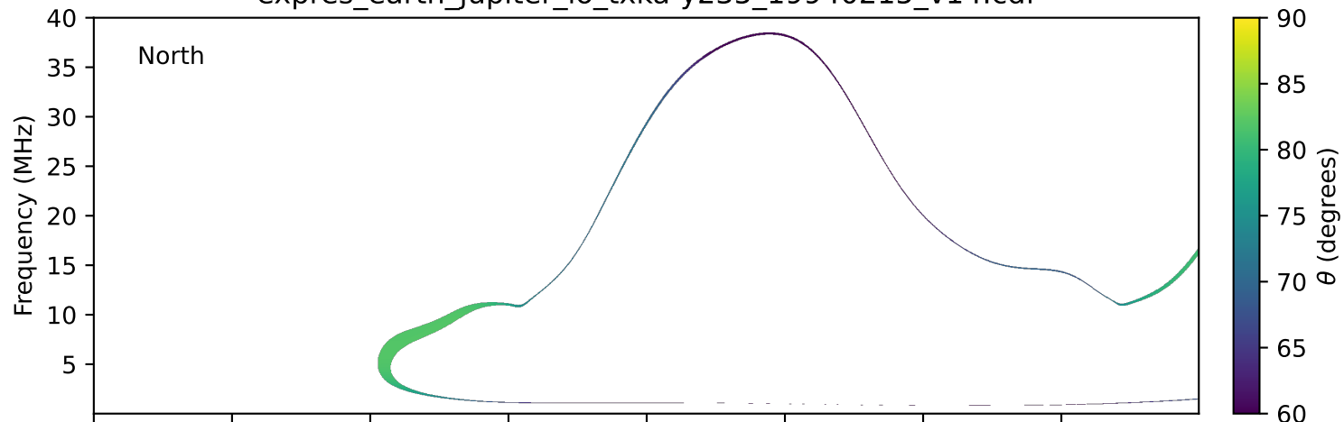
expres_earth_jupiter_io_txka-y235_19940215_v14.cdf
