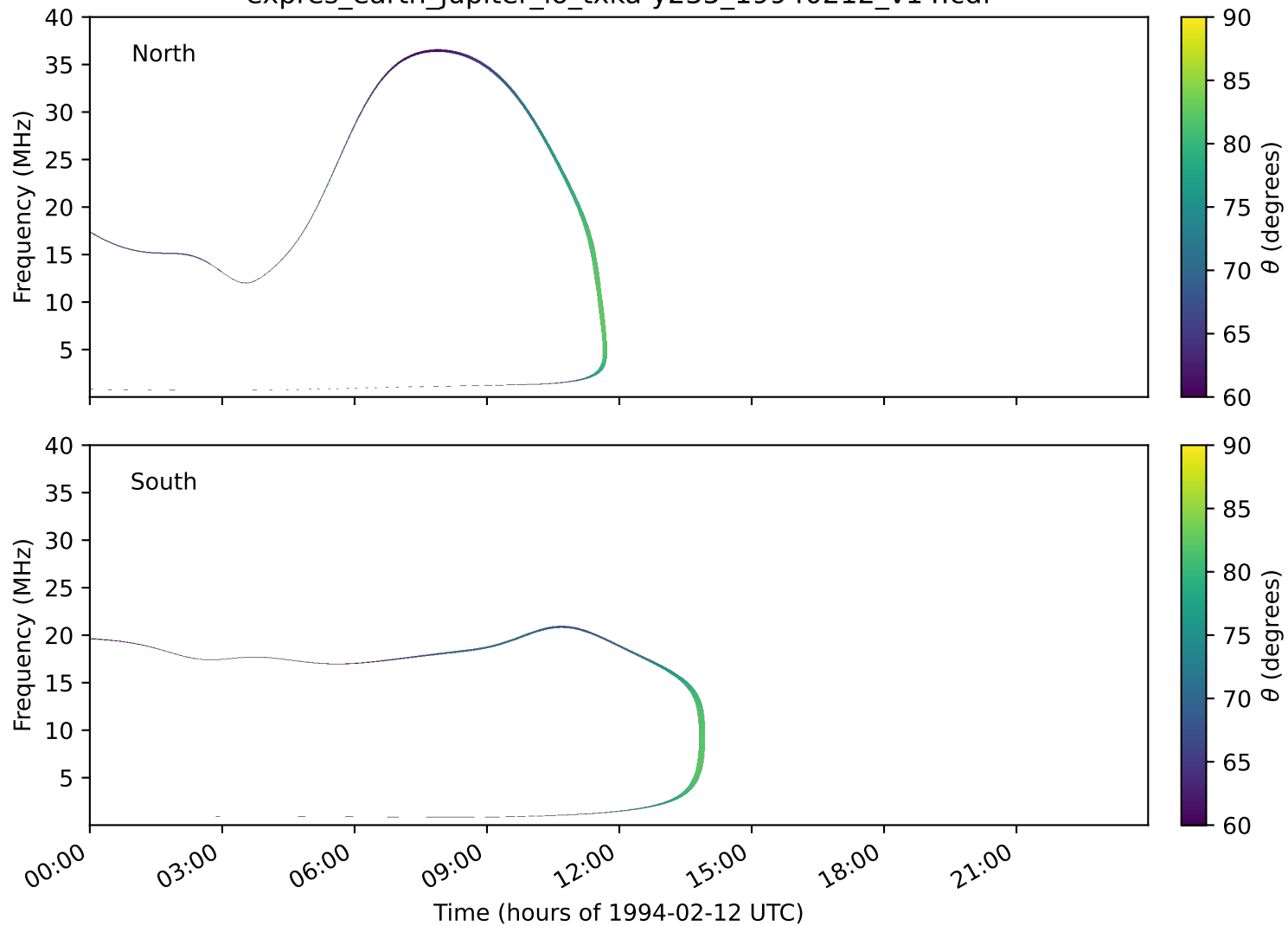
expres_earth_jupiter_io_txka-y235_19940212_v14.cdf
