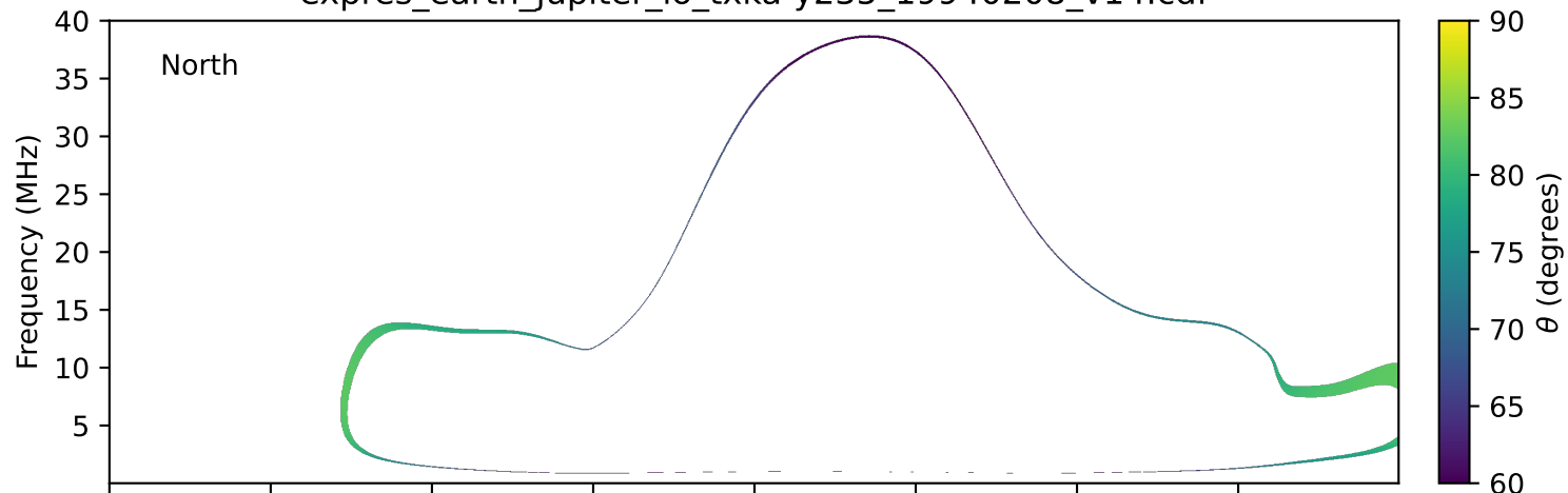
expres_earth_jupiter_io_txka-y235_19940208_v14.cdf
