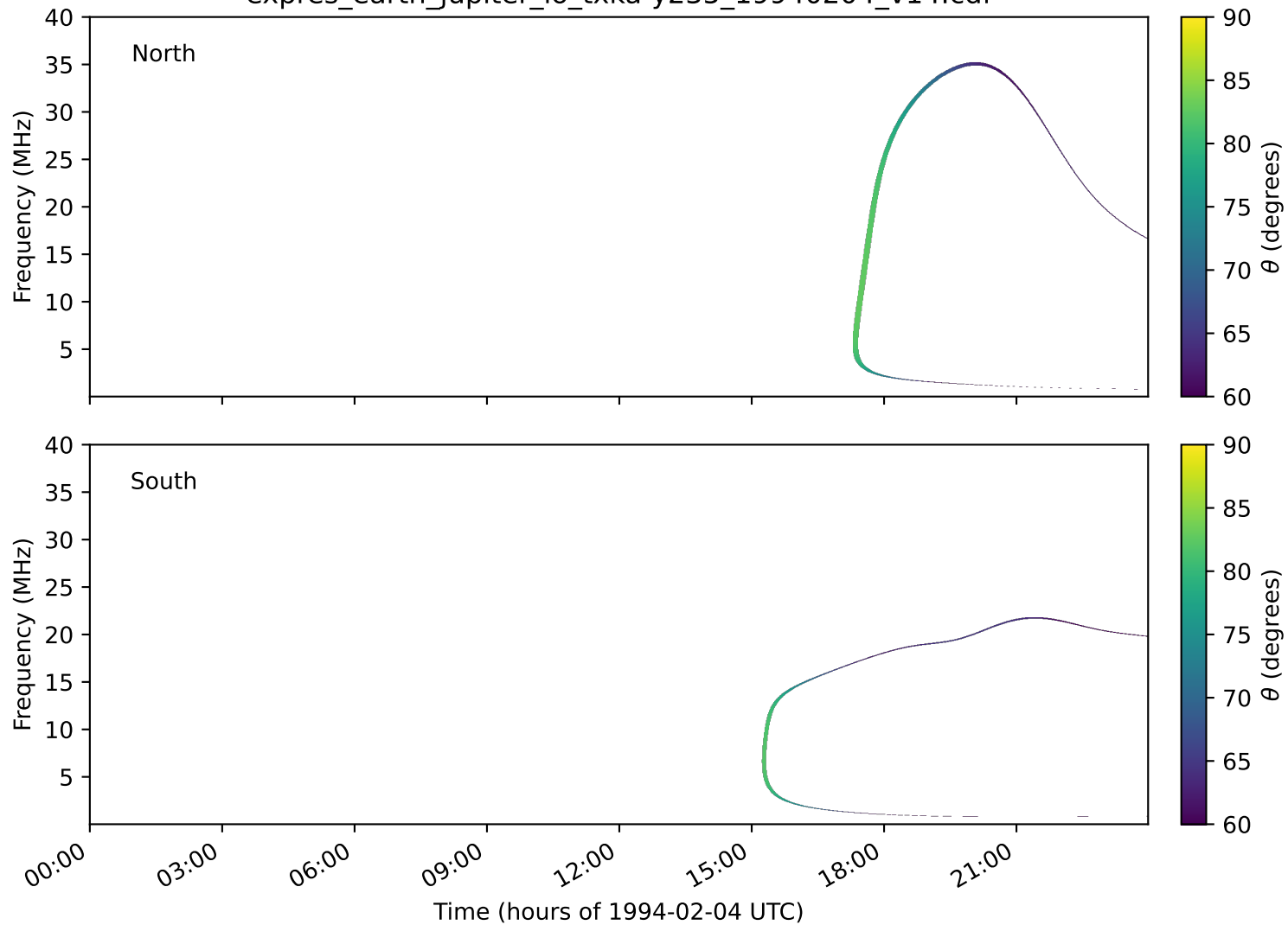
expres_earth_jupiter_io_txka-y235_19940204_v14.cdf
