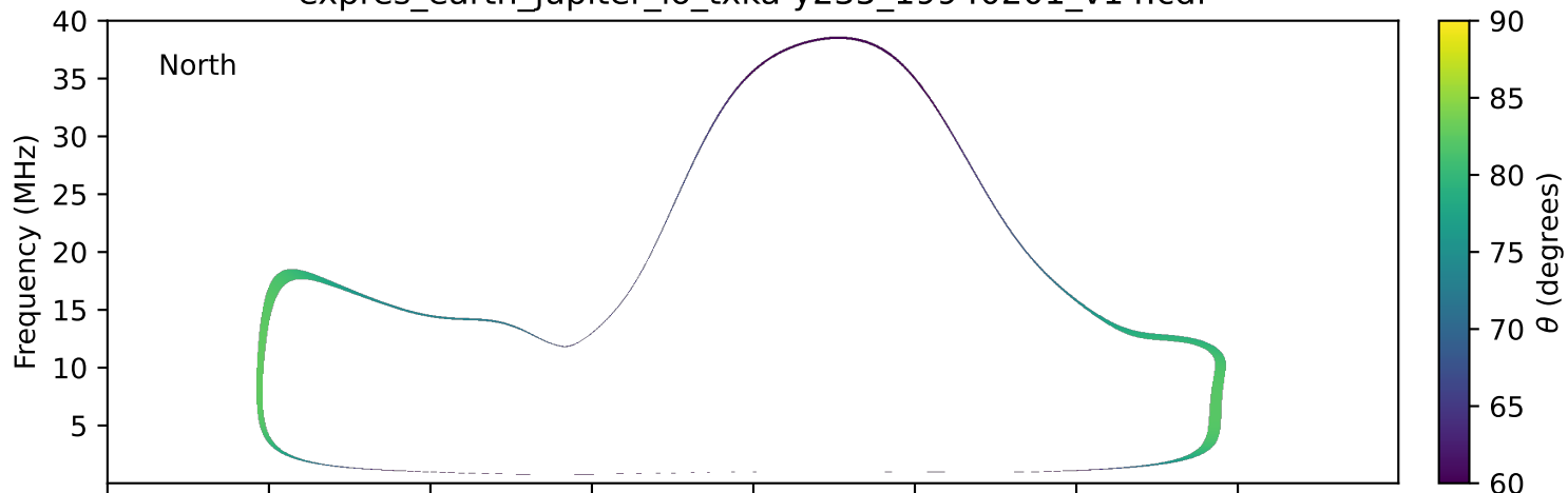
expres_earth_jupiter_io_txka-y235_19940201_v14.cdf
