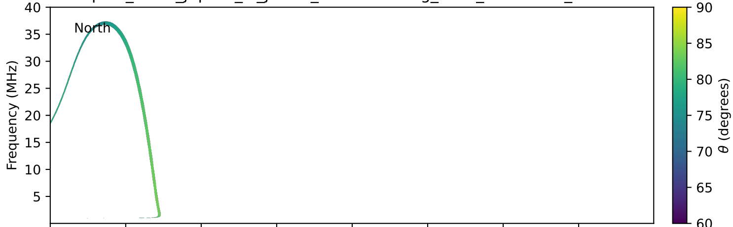
expres_earth_jupiter_io_jrm33_lossc-wid1deg_3kev_19940223_v11.cdf
