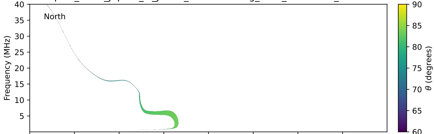
expres_earth_jupiter_io_jrm33_lossc-wid1deg_3kev_19940221_v11.cdf
