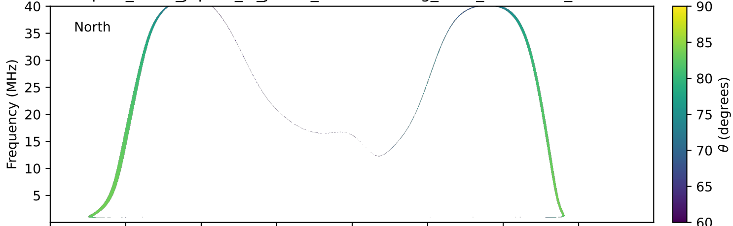
expres_earth_jupiter_io_jrm33_lossc-wid1deg_3kev_19940217_v11.cdf
