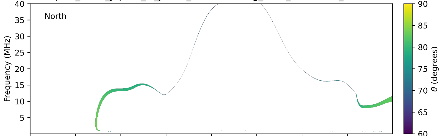
expres_earth_jupiter_io_jrm33_lossc-wid1deg_3kev_19940208_v11.cdf
