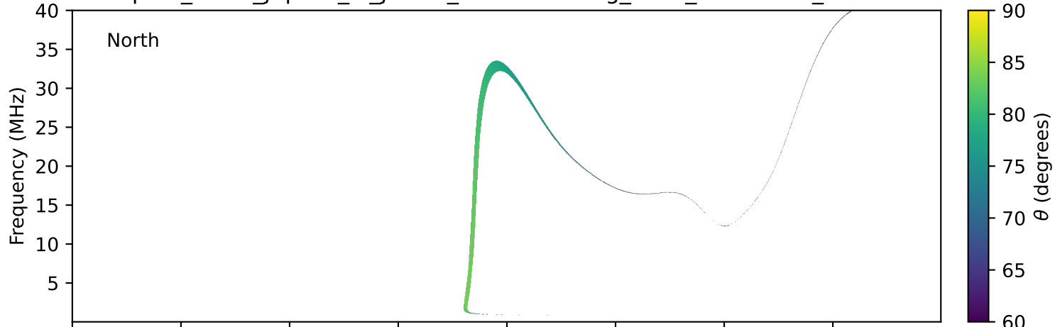
expres_earth_jupiter_io_jrm33_lossc-wid1deg_3kev_19940206_v11.cdf
