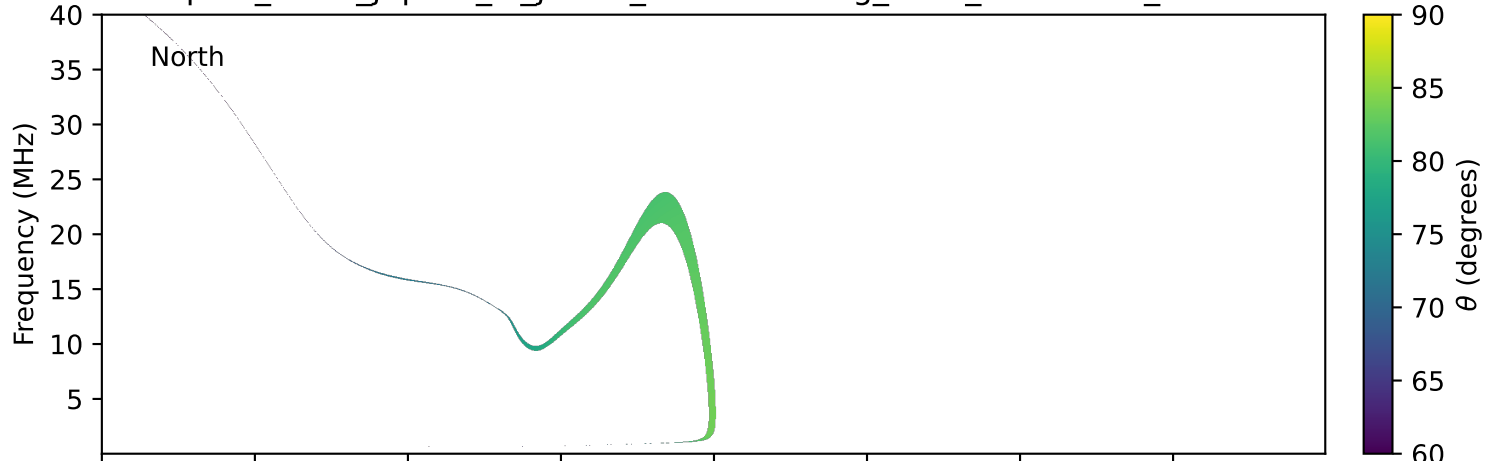
expres_earth_jupiter_io_jrm09_lossc-wid1deg_3kev_19940228_v11.cdf
