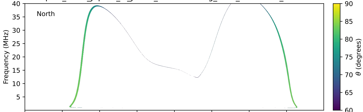
expres_earth_jupiter_io_jrm09_lossc-wid1deg_3kev_19940224_v11.cdf
