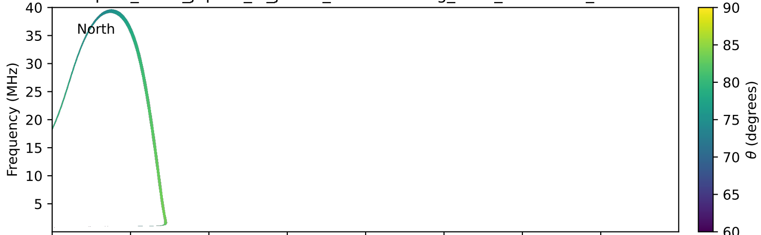
expres_earth_jupiter_io_jrm09_lossc-wid1deg_3kev_19940223_v11.cdf
