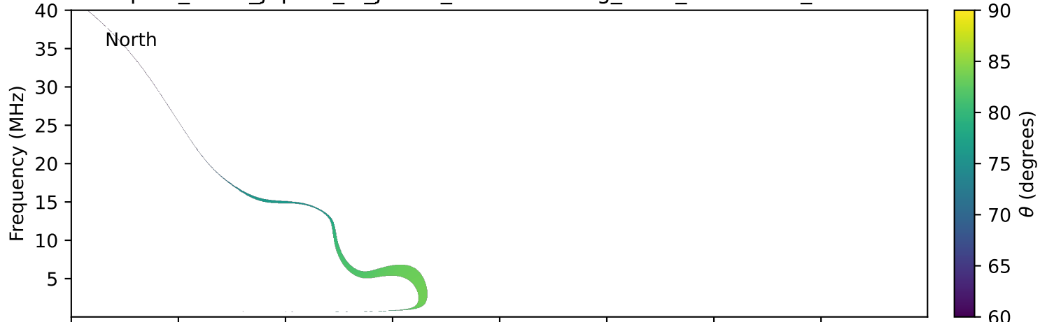
expres_earth_jupiter_io_jrm09_lossc-wid1deg_3kev_19940221_v11.cdf
