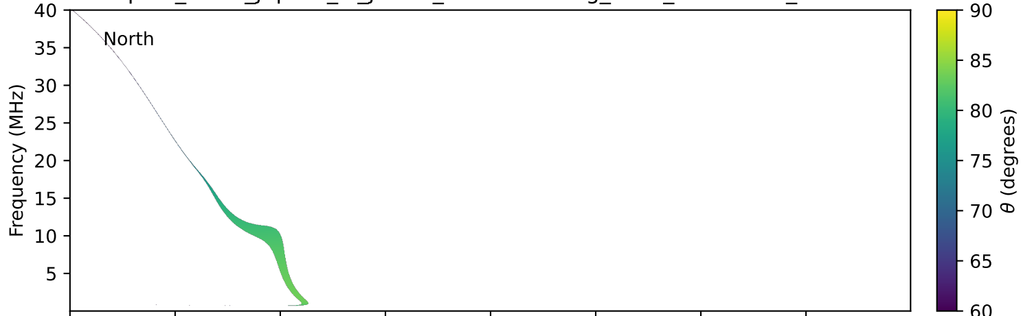
expres_earth_jupiter_io_jrm09_lossc-wid1deg_3kev_19940214_v11.cdf
