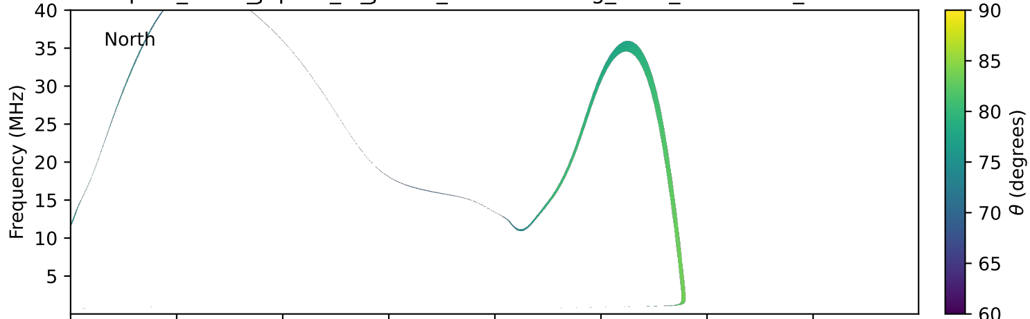
expres_earth_jupiter_io_jrm09_lossc-wid1deg_3kev_19940203_v11.cdf
