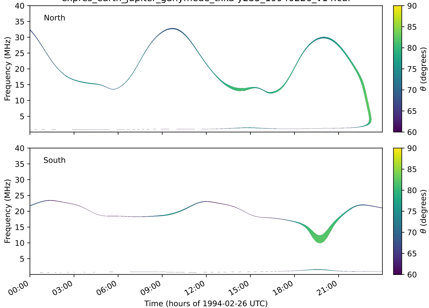
expres_earth_jupiter_ganymede_txka-y235_19940226_v14.cdf
