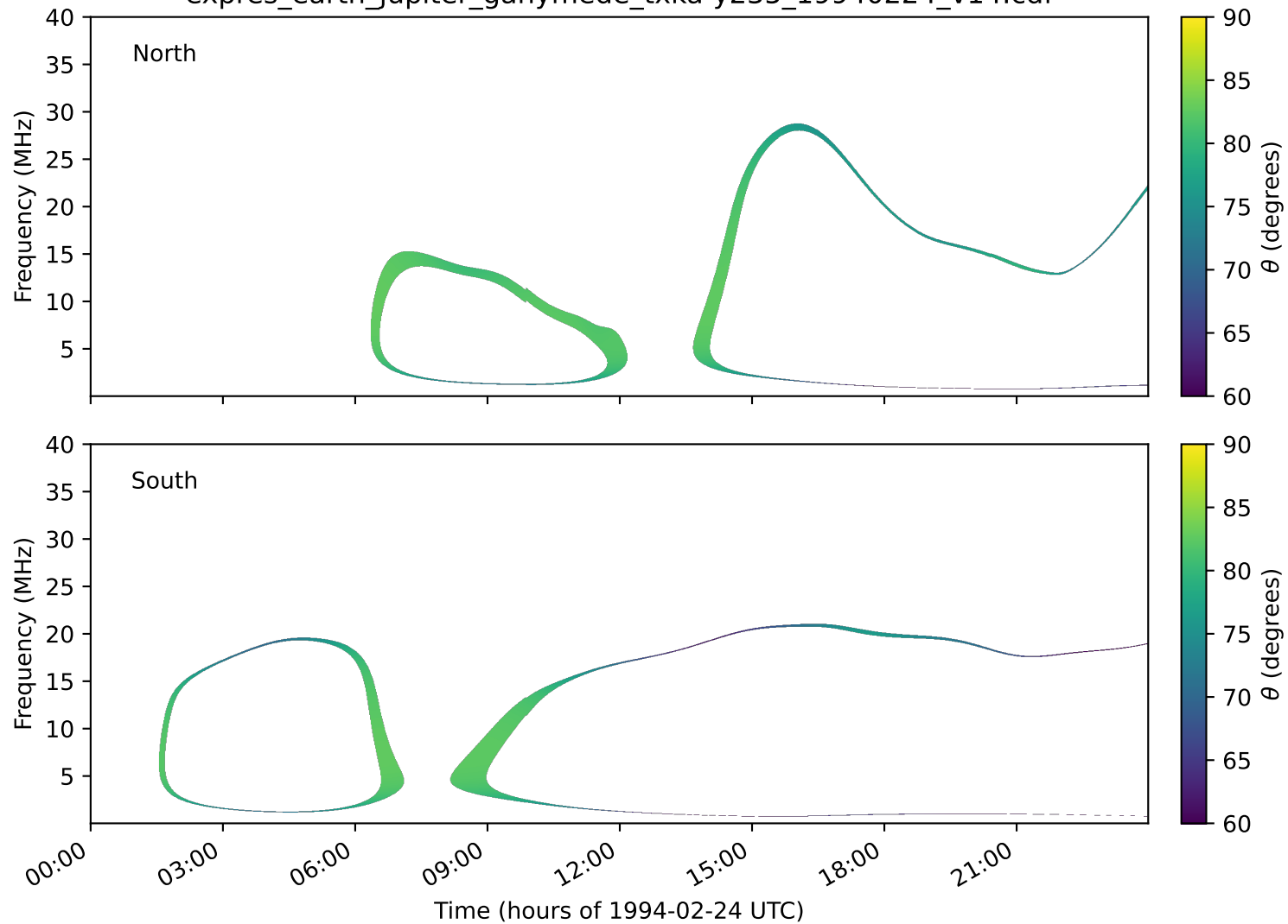
expres_earth_jupiter_ganymede_txka-y235_19940224_v14.cdf
