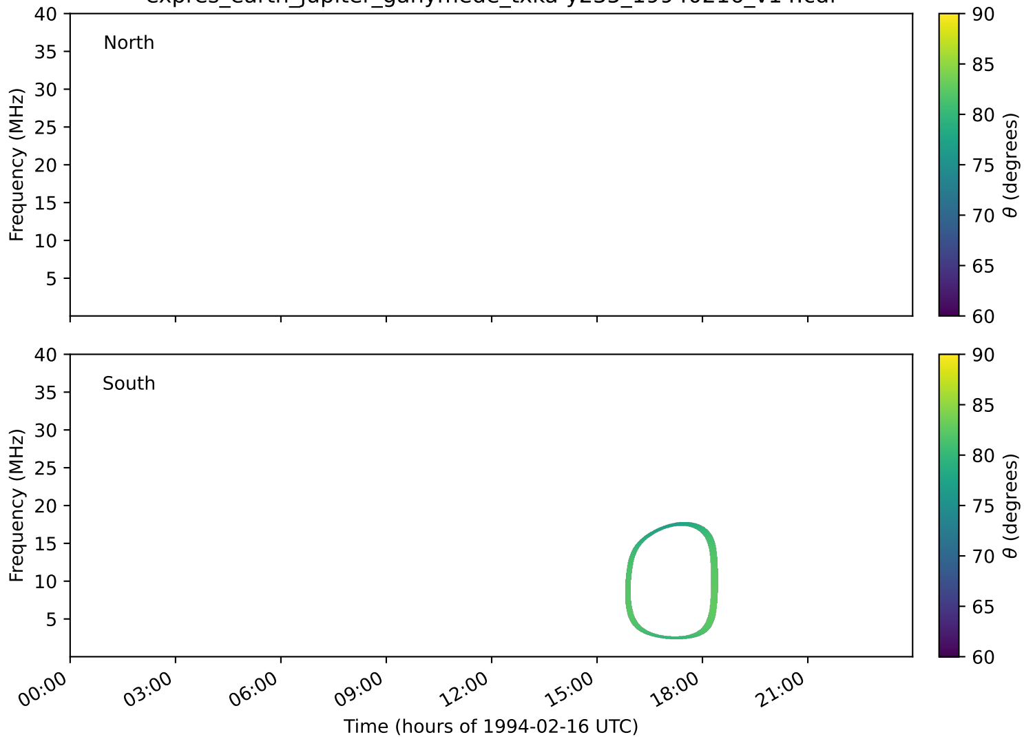
expres_earth_jupiter_ganymede_txka-y235_19940216_v14.cdf
