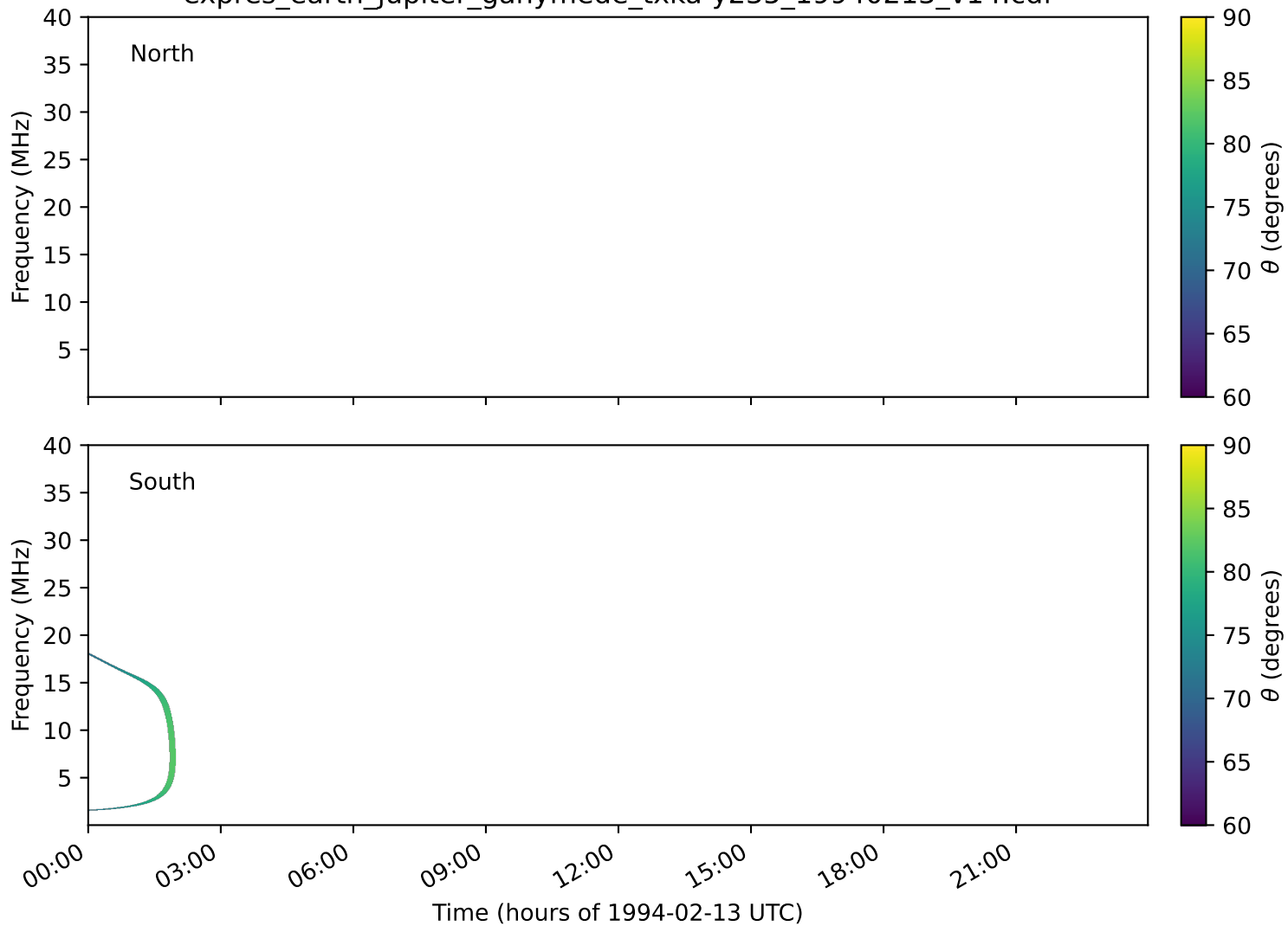
expres_earth_jupiter_ganymede_txka-y235_19940213_v14.cdf
