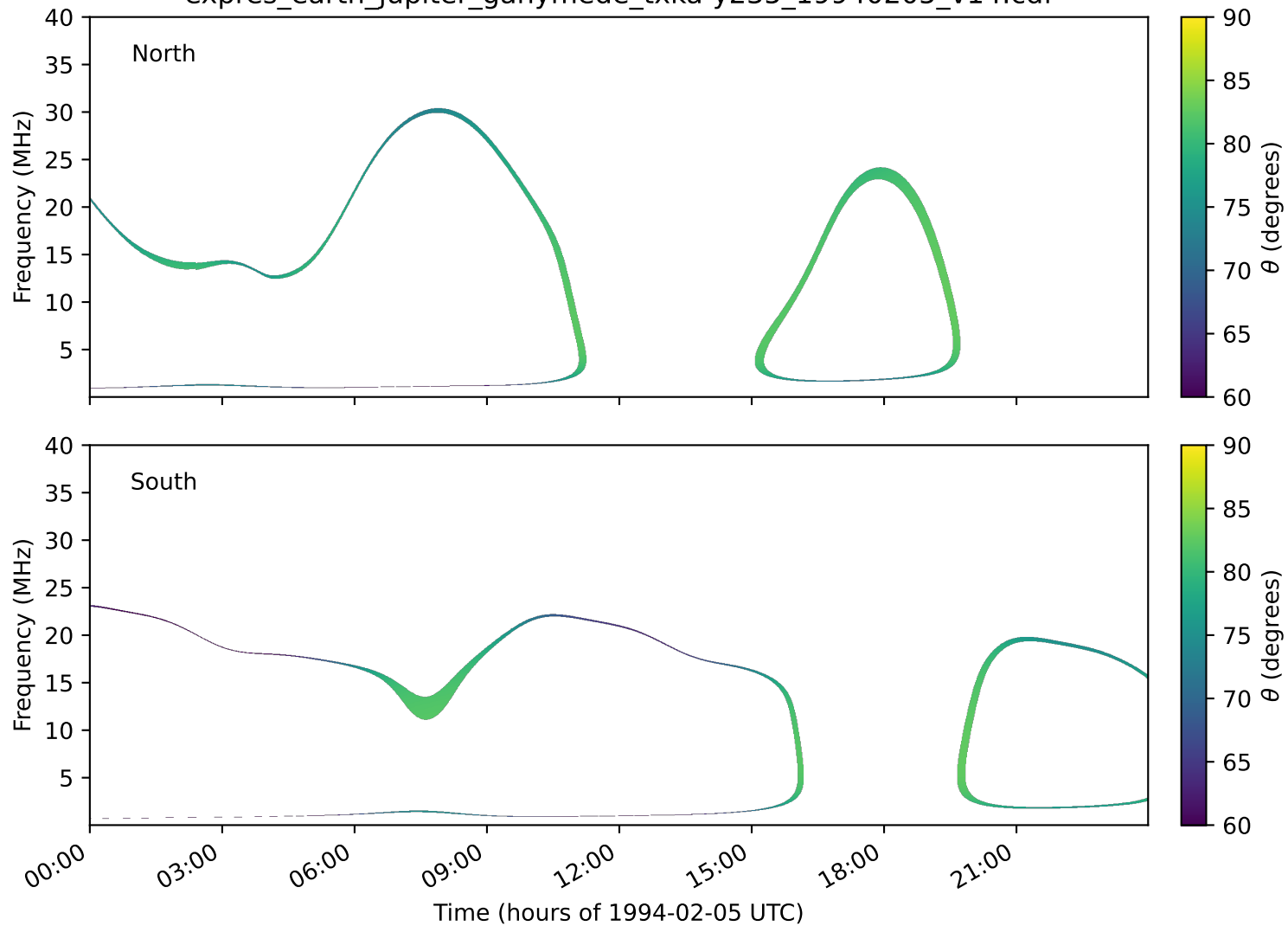
expres_earth_jupiter_ganymede_txka-y235_19940205_v14.cdf
