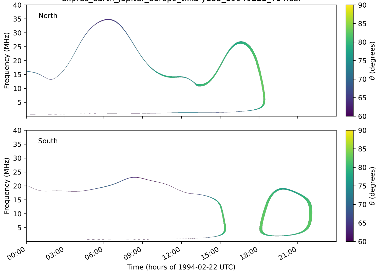
expres_earth_jupiter_europa_txka-y235_19940222_v14.cdf
