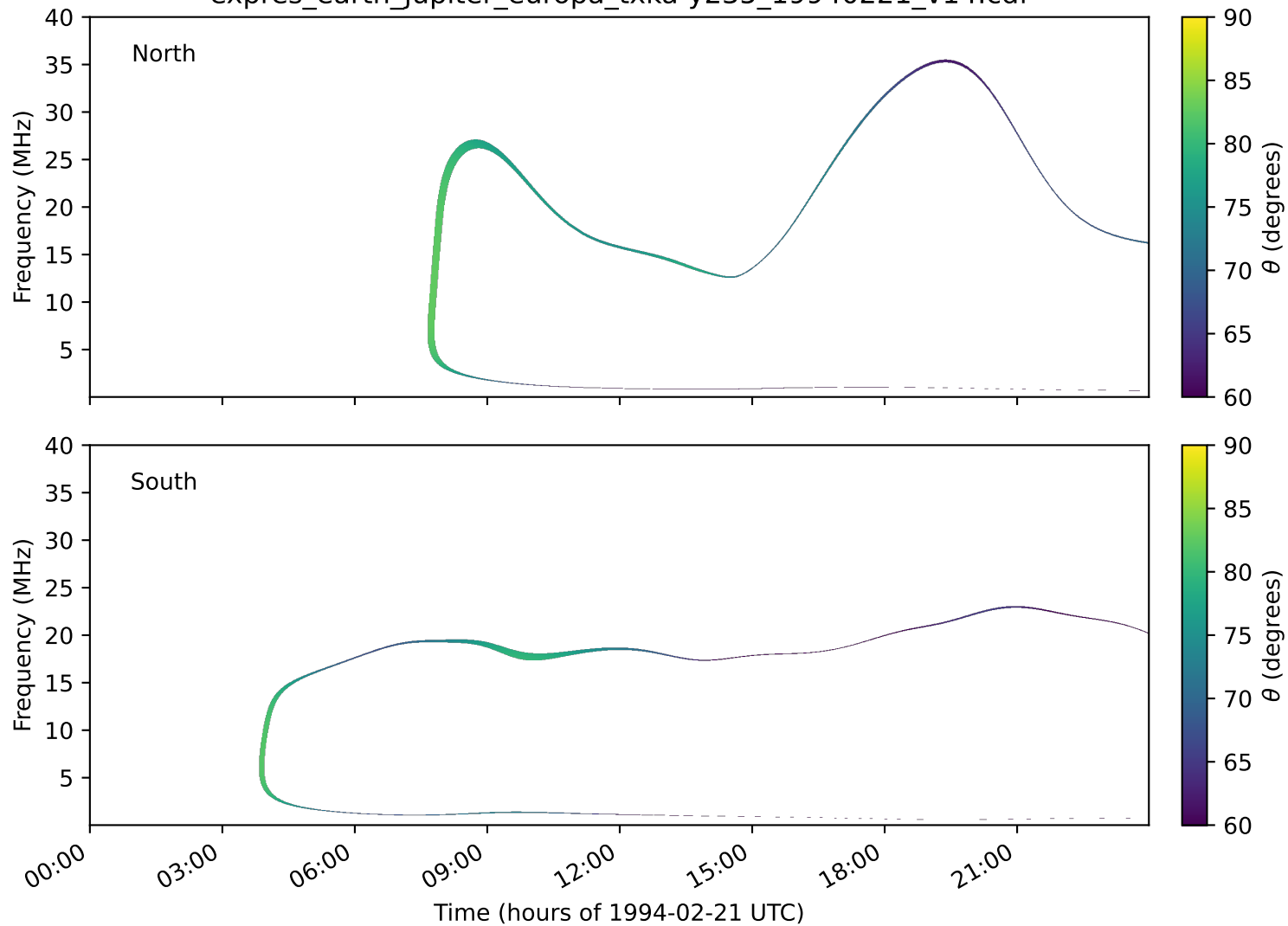
expres_earth_jupiter_europa_txka-y235_19940221_v14.cdf
