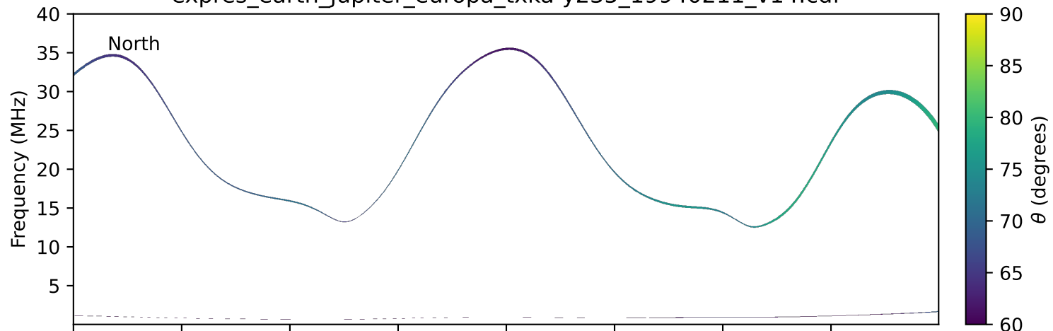
expres_earth_jupiter_europa_txka-y235_19940211_v14.cdf
