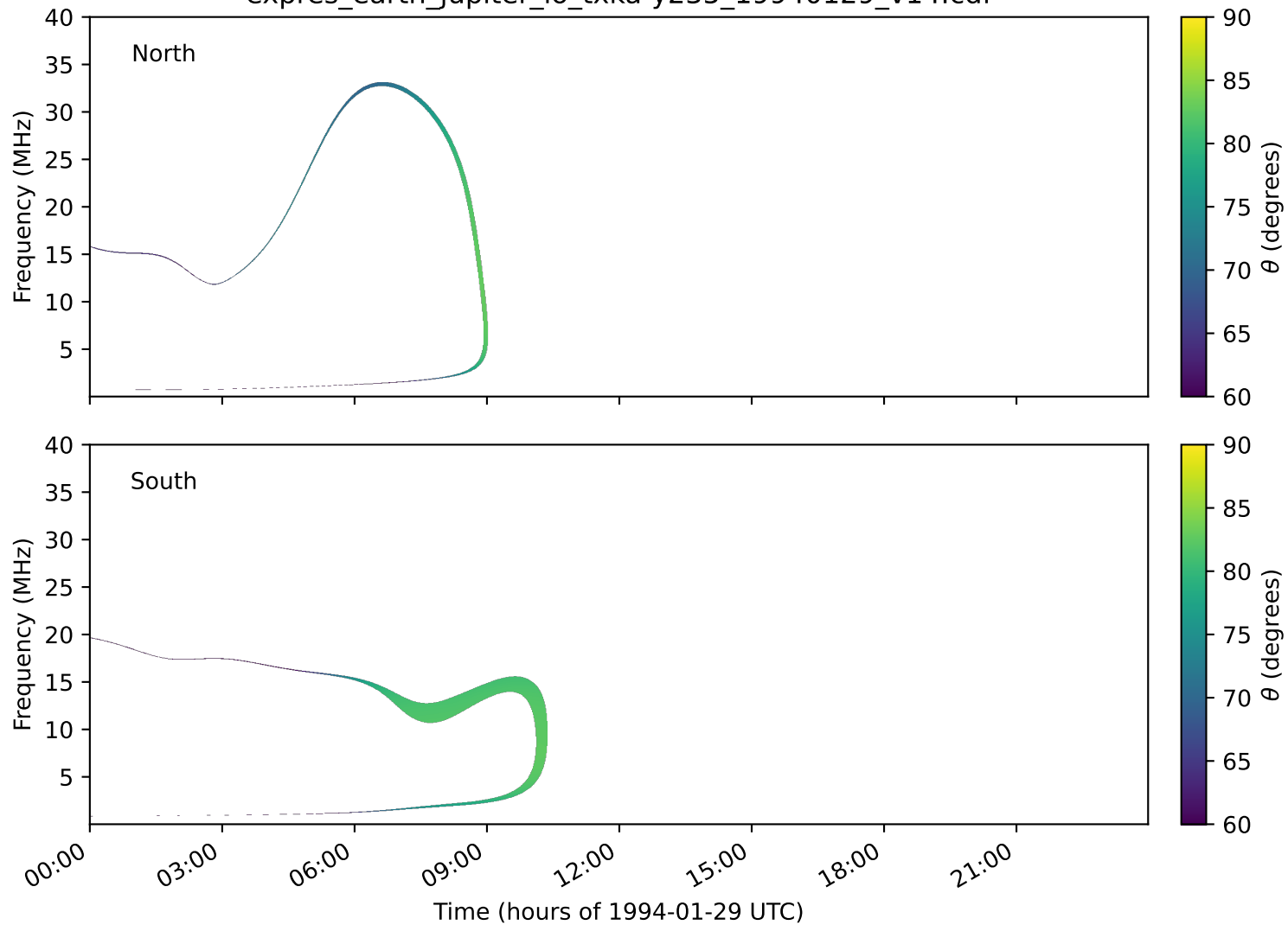
expres_earth_jupiter_io_txka-y235_19940129_v14.cdf
