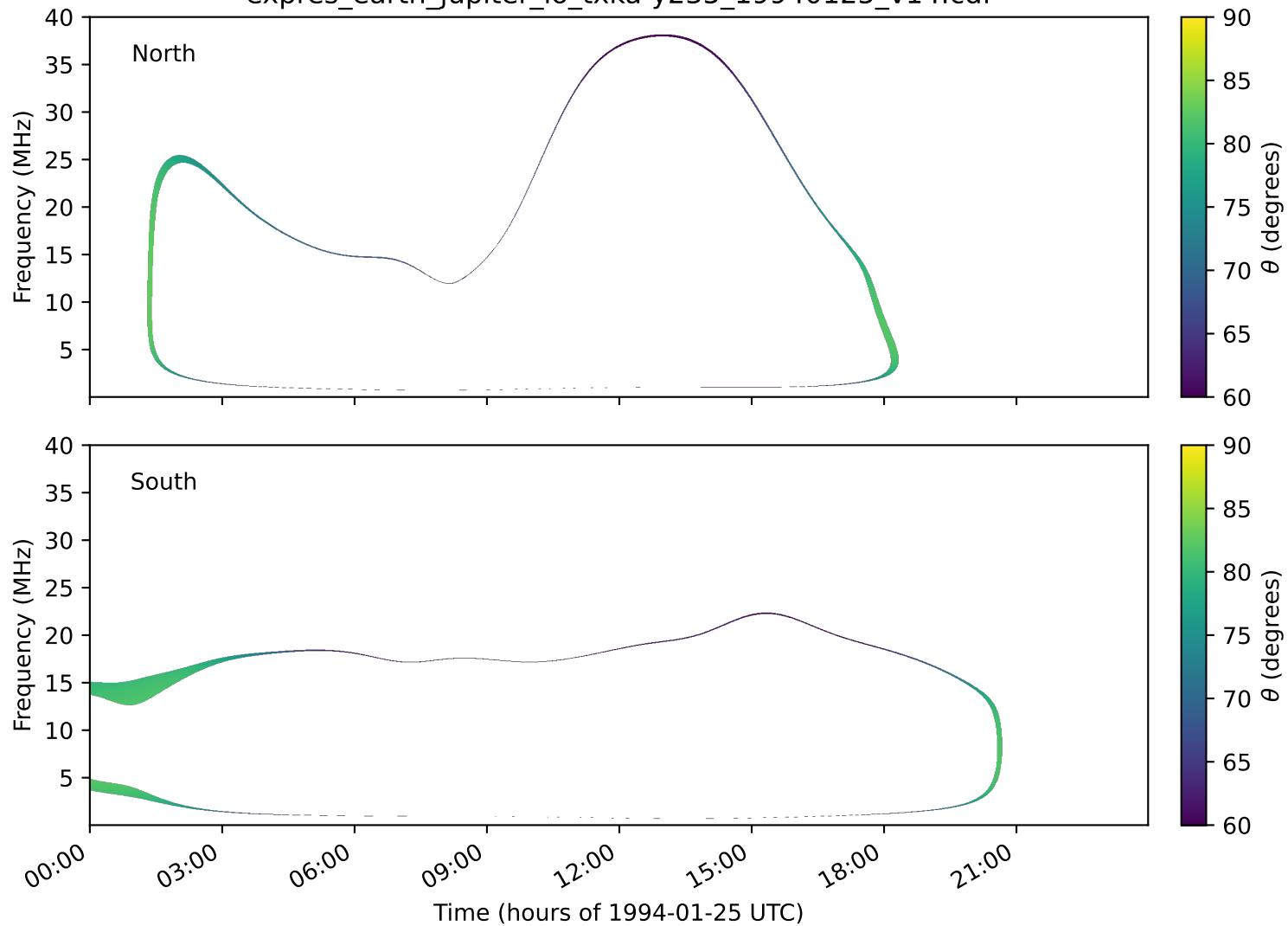
expres_earth_jupiter_io_txka-y235_19940125_v14.cdf
