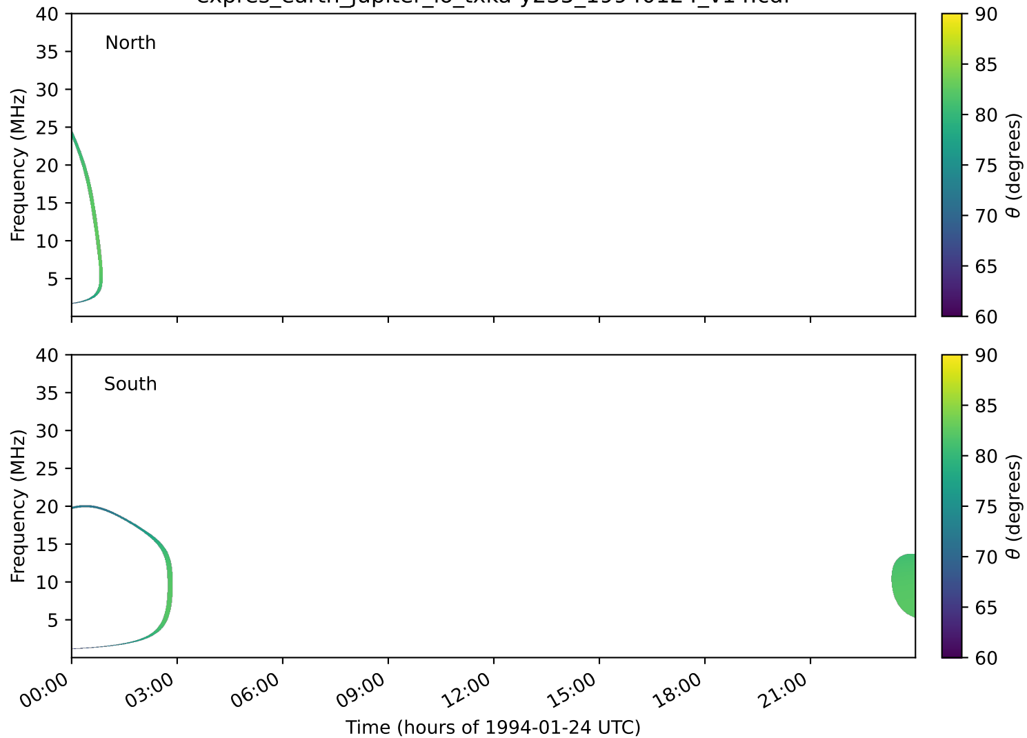
expres_earth_jupiter_io_txka-y235_19940124_v14.cdf
