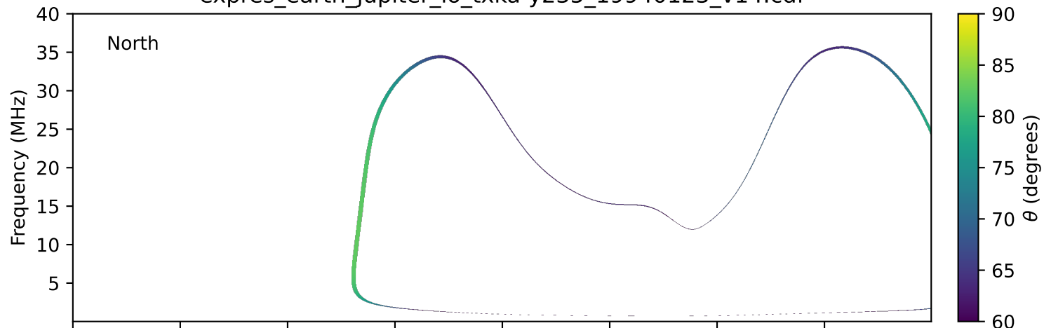
expres_earth_jupiter_io_txka-y235_19940123_v14.cdf
