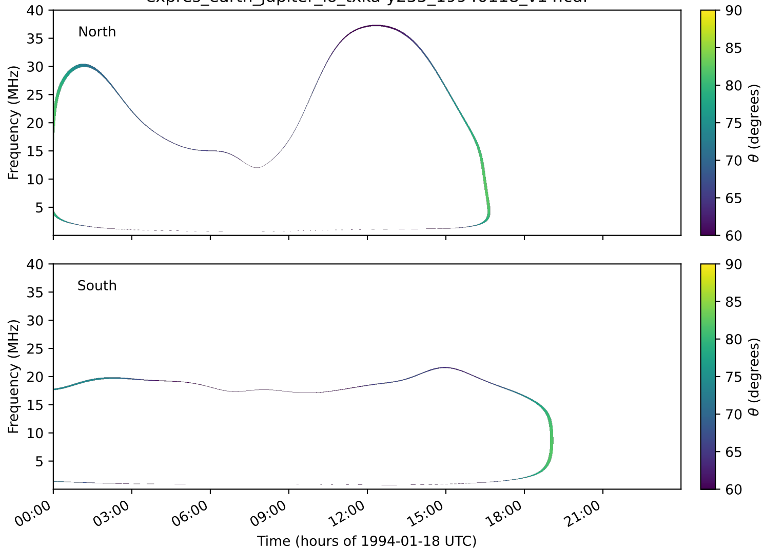
expres_earth_jupiter_io_txka-y235_19940118_v14.cdf
