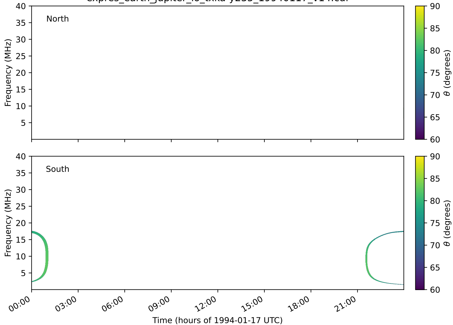
expres_earth_jupiter_io_txka-y235_19940117_v14.cdf
