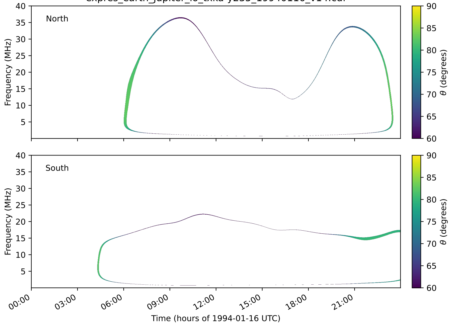
expres_earth_jupiter_io_txka-y235_19940116_v14.cdf
