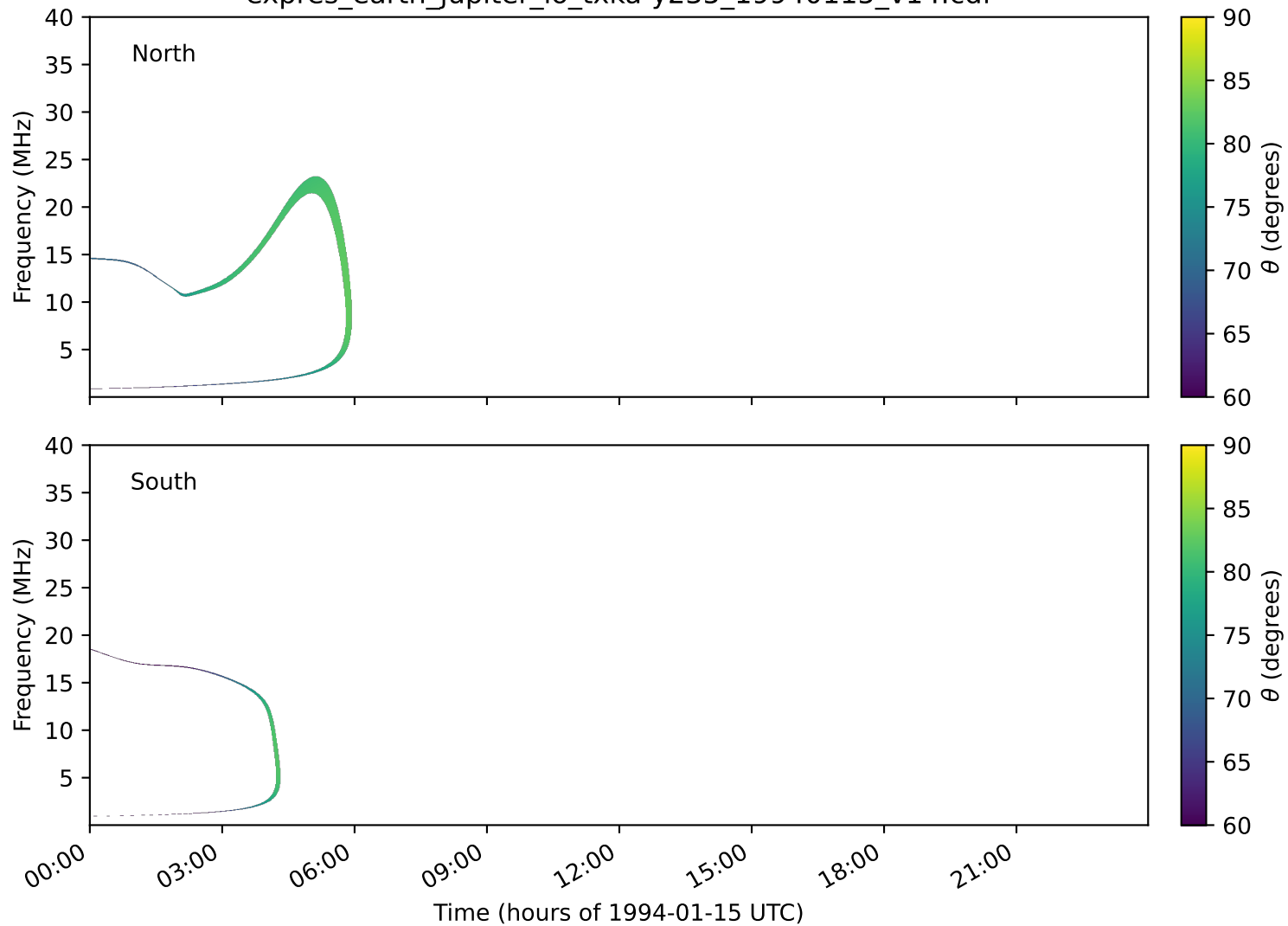
expres_earth_jupiter_io_txka-y235_19940115_v14.cdf
