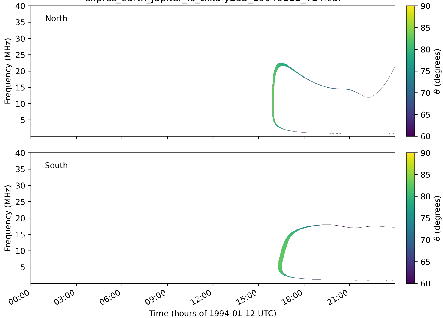
expres_earth_jupiter_io_txka-y235_19940112_v14.cdf
