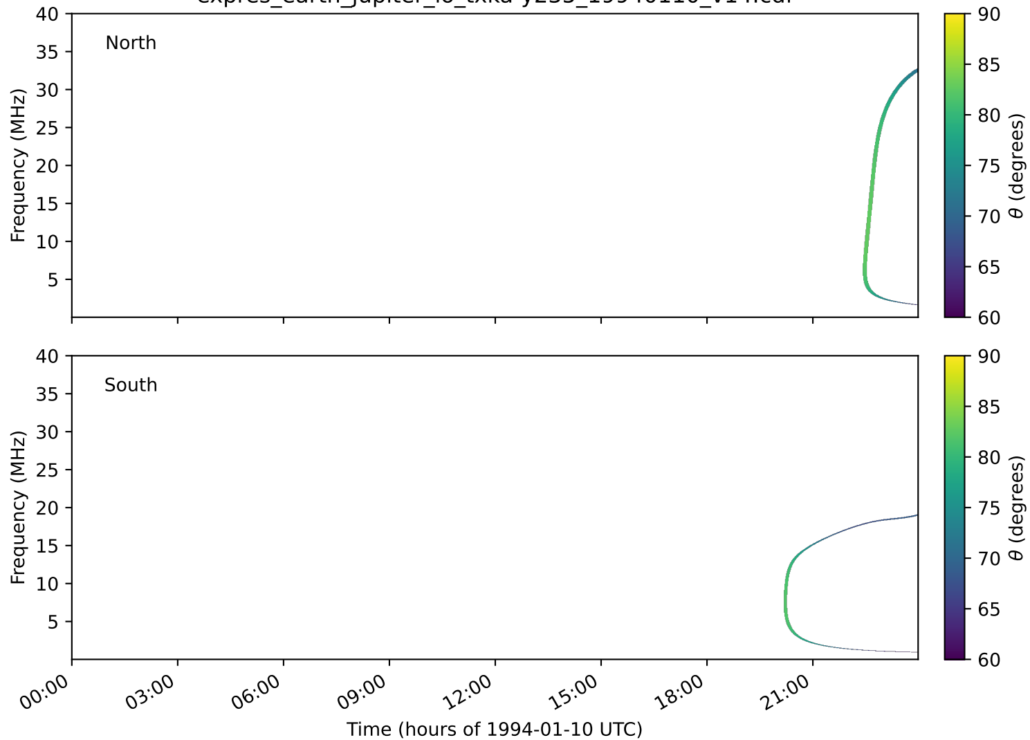
expres_earth_jupiter_io_txka-y235_19940110_v14.cdf
