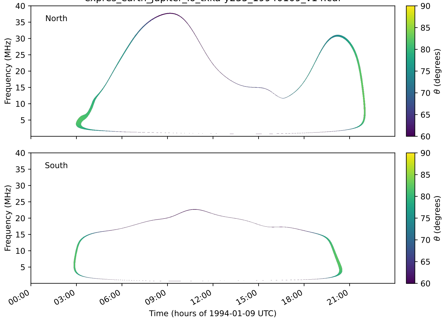
expres_earth_jupiter_io_txka-y235_19940109_v14.cdf
