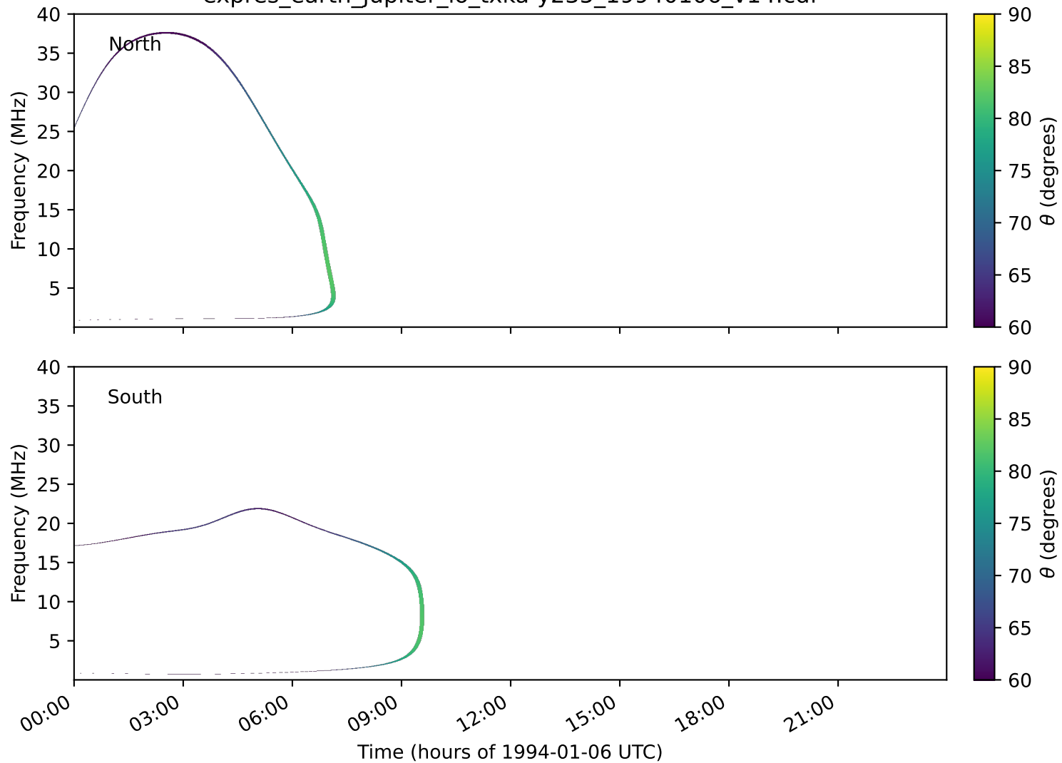
expres_earth_jupiter_io_txka-y235_19940106_v14.cdf
