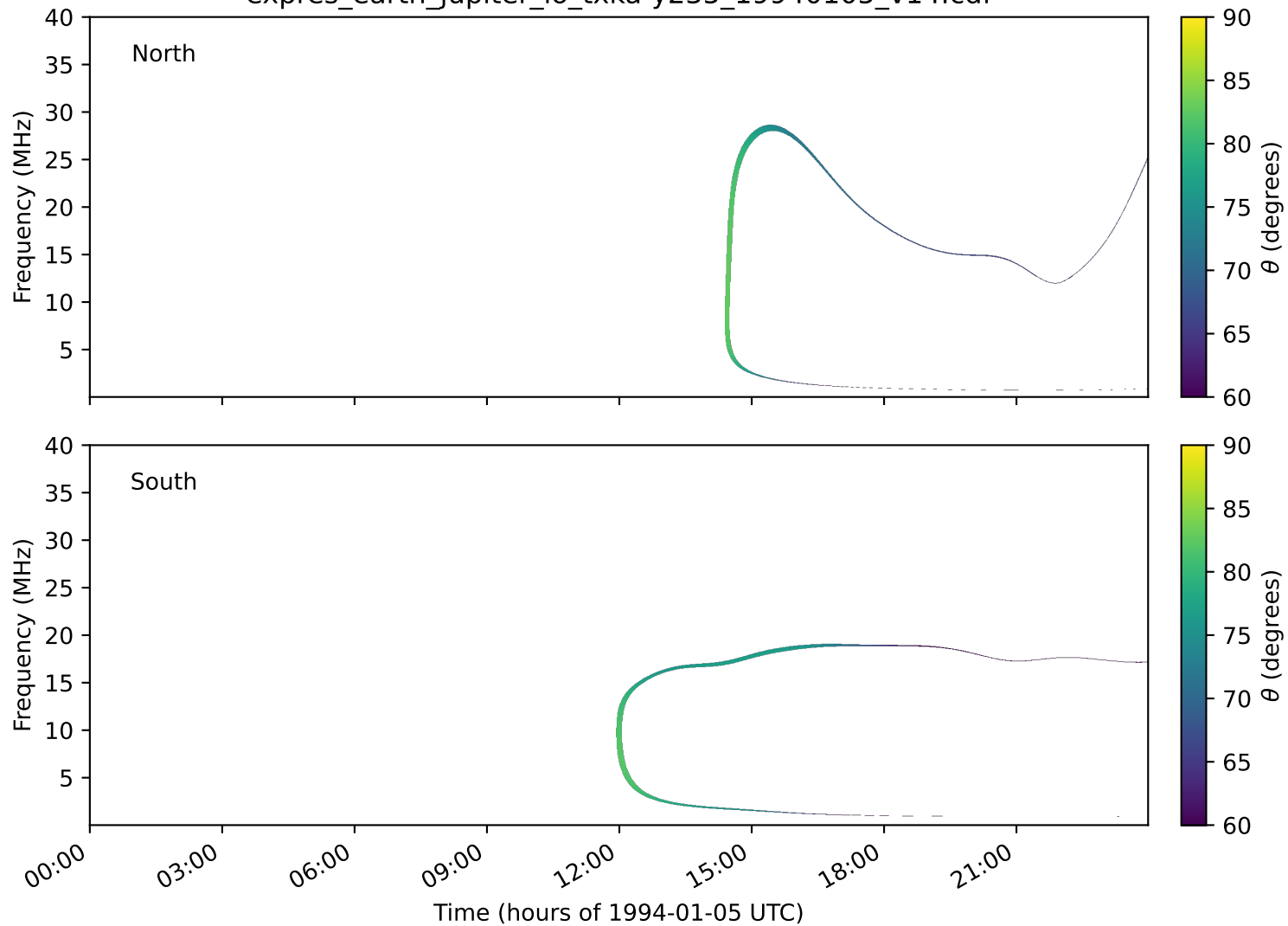
expres_earth_jupiter_io_txka-y235_19940105_v14.cdf
