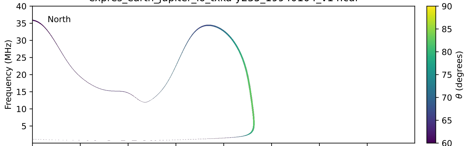
expres_earth_jupiter_io_txka-y235_19940104_v14.cdf
