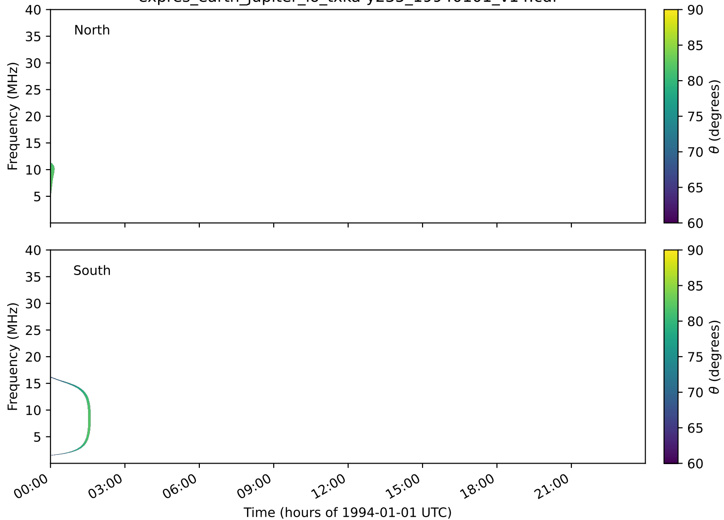
expres_earth_jupiter_io_txka-y235_19940101_v14.cdf
