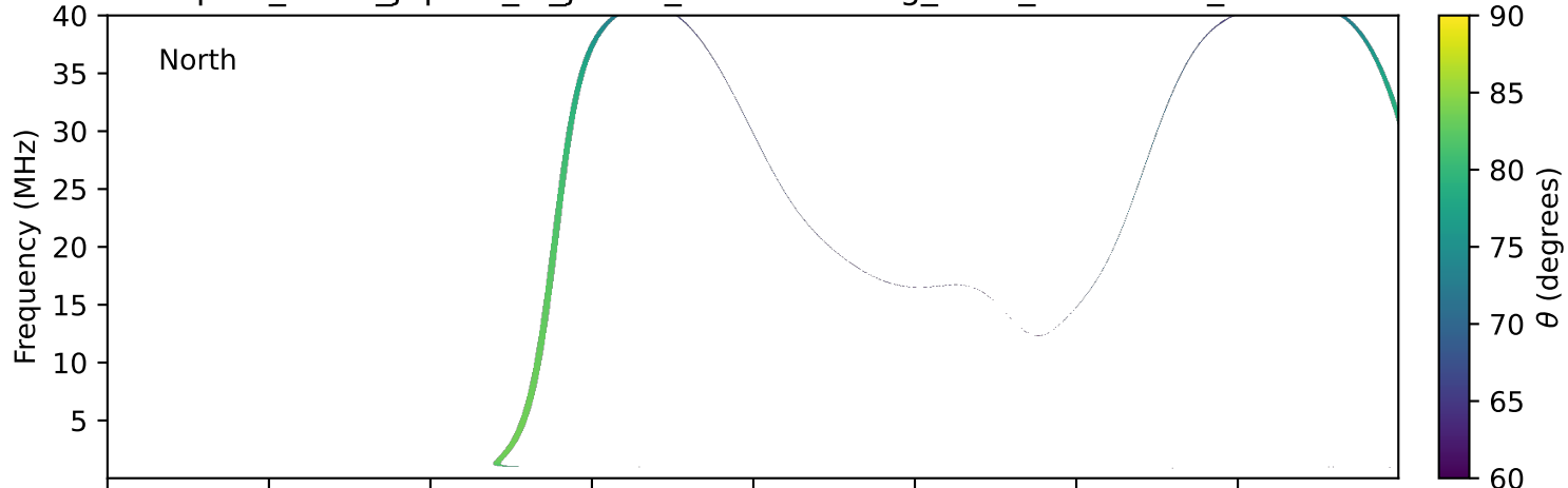
expres_earth_jupiter_io_jrm33_lossc-wid1deg_3kev_19940123_v11.cdf
